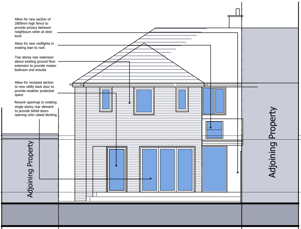
REAR ELEVATION (South)
