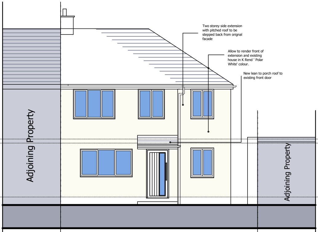
FRONT ELEVATION (North)
